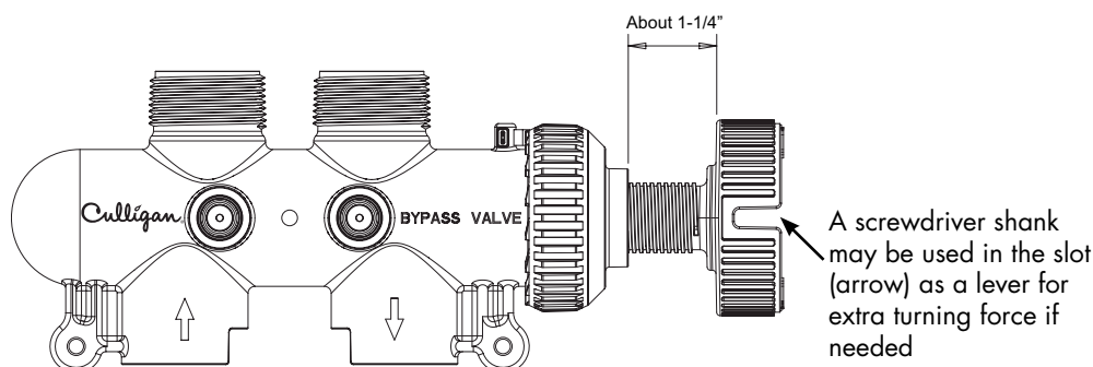
Figure 24. Bypass valve.
